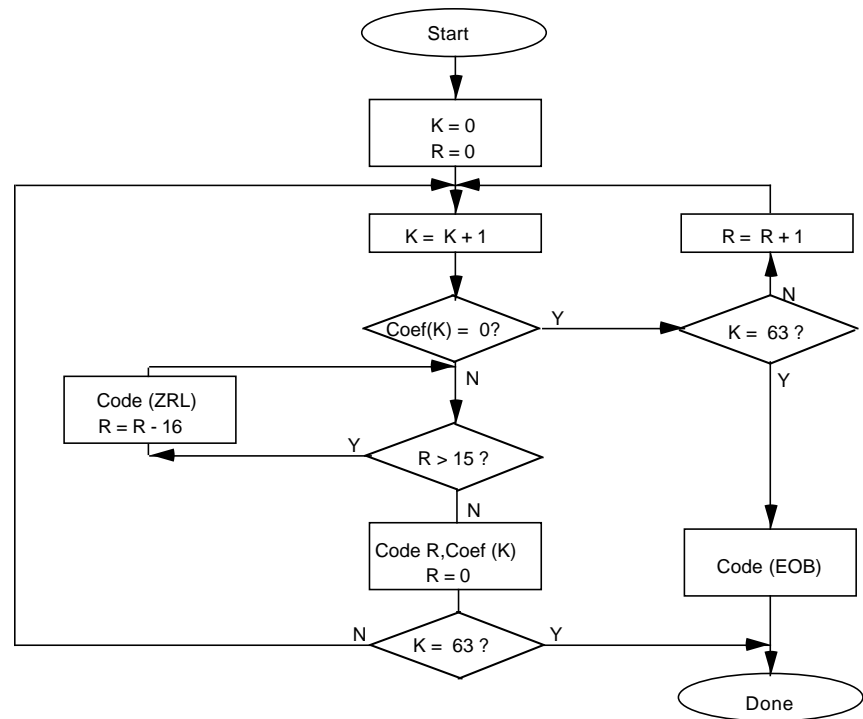
Figure 5. Encoding Procedure for AC Coeffs
